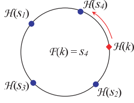
Figure 1: Keys are consistently hashed onto resolver switches ( s_i ).
