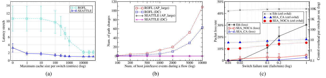
Figure 5: (a) Stretch across different cache sizes in AP-large with 10K hosts (b) Path stability (c) Effect of switch failures in DC .
