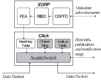
Figure 7: Implementation architecture.
